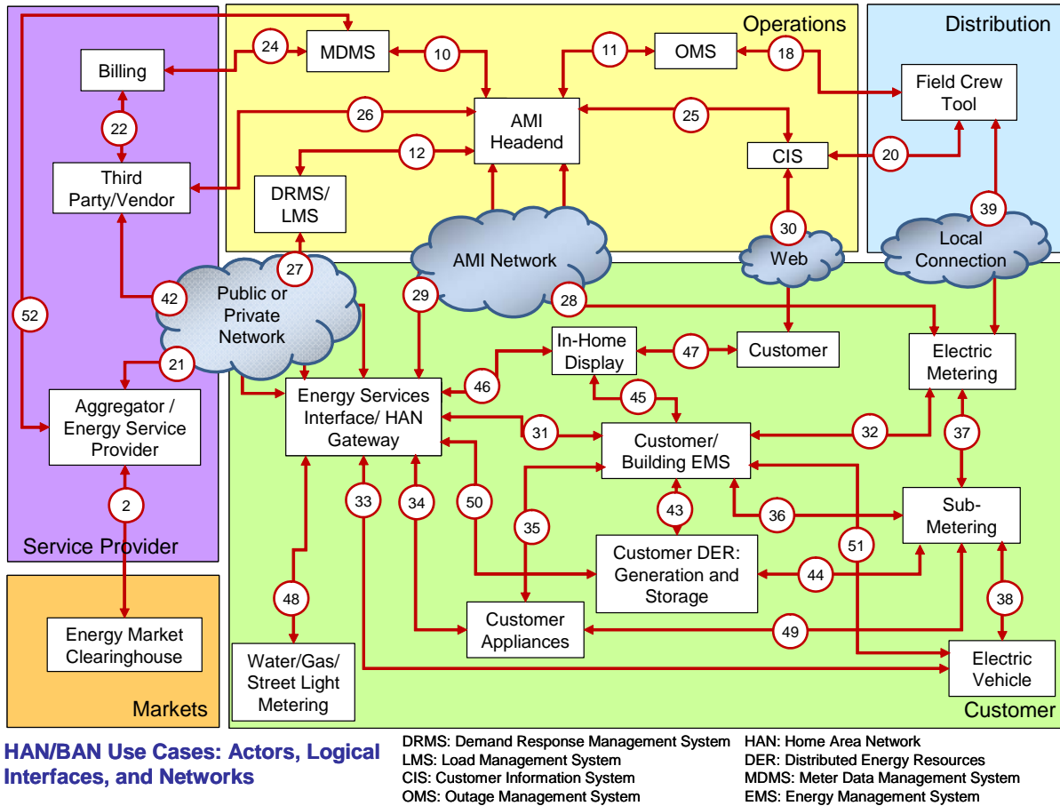
Figure 2: HAN/BAN Actors, Logical Interfaces, and Networks
