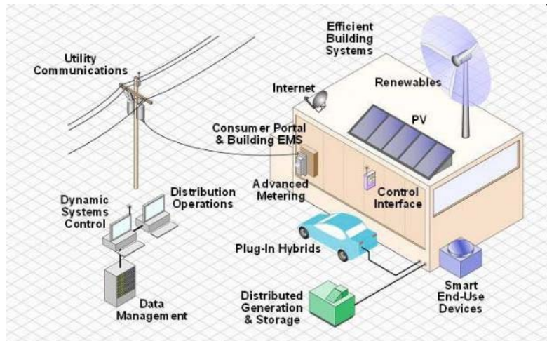
Figure 1: Home Area Network (HAN) Appliances and Equipment ( credit EPRI )
