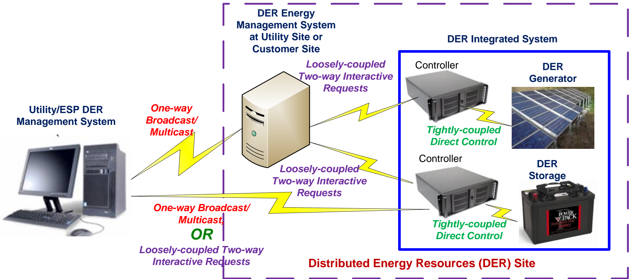
DER Management: Interactions between Components
